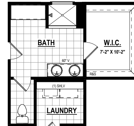
PRIMARY BATH W/ MAKEUP VANITY Option #60905
