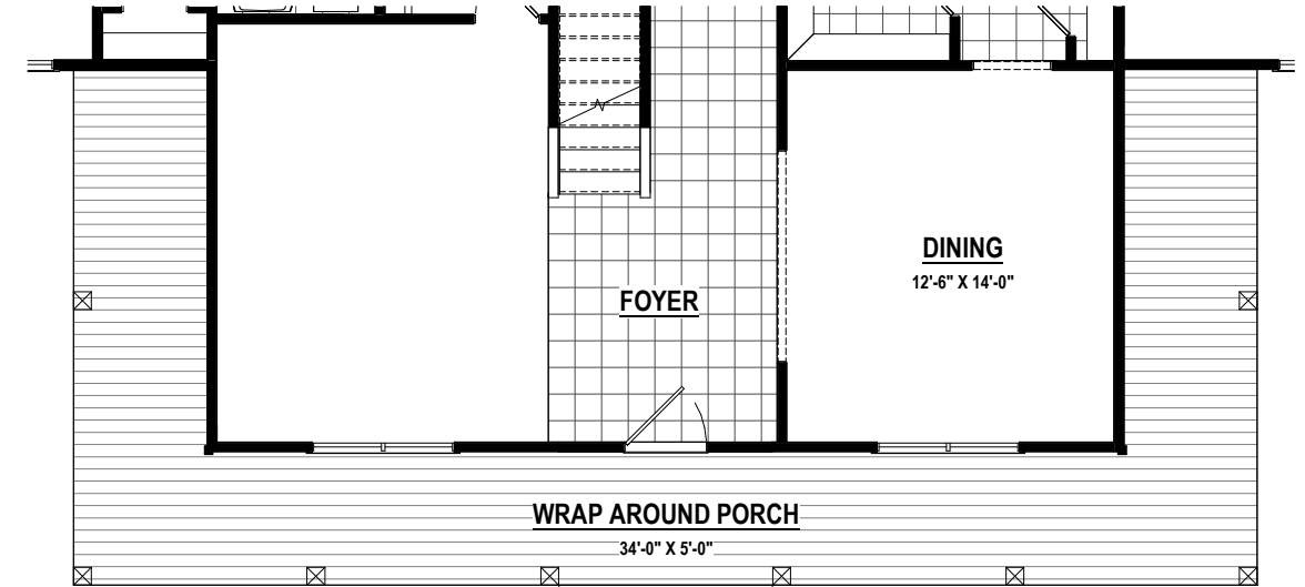
WRAP AROUND PORCH (180 SF ±) Option # 15246
