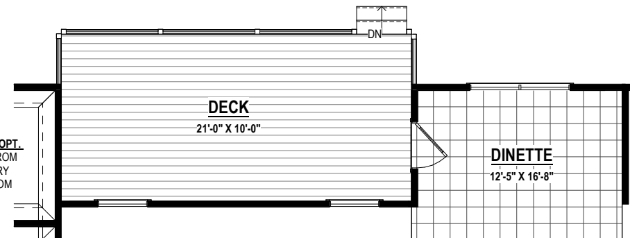
WOOD DECK W/ DINETTE EXTENSION (144 SF ± 84 SF ±) Option # 15007 Option # 15017 Option # 15125 Option # 15126
