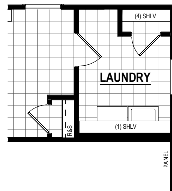
LAUNDRY W/ CLOSET 8' Option # 15040 9' Option # 15041
