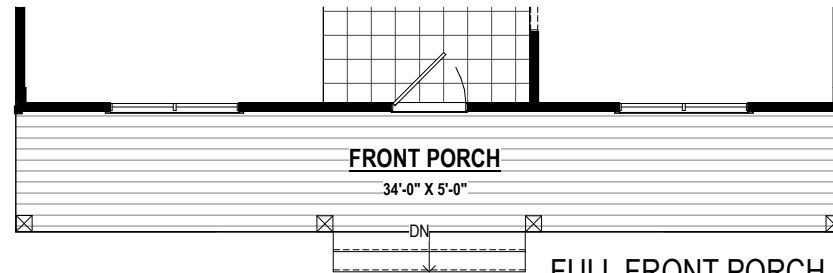
FULL FRONT PORCH (180 SF ±) Option # 15240
