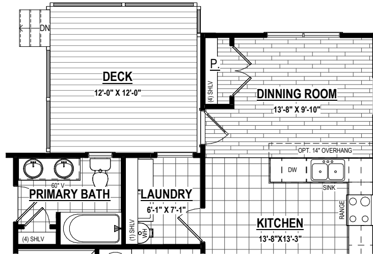
DINETTE W/ DECK (128 SF ±)
